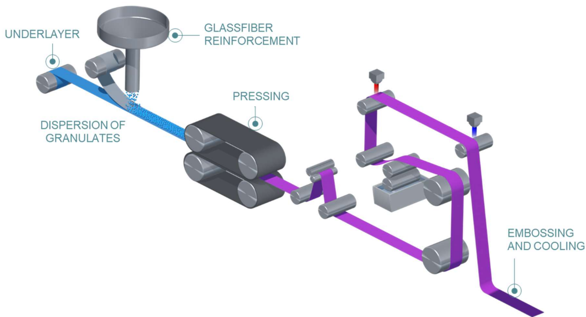
Pressing manufacturing process flow diagram
